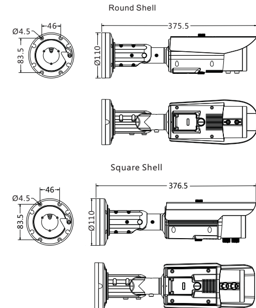
Figure 2-3 Dimensions ( Unit:mm )
