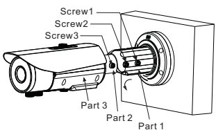
Figure 3-3 Loosening screws
