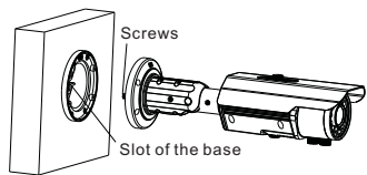
Figure 3-1 Installing camera
